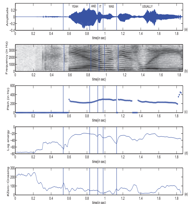
Fig. 1. An example speech utterance to illustrate the limitations of the acoustic features in detecting word boundaries: (a) time signal (b) spectrogram (c) short-time pitch (d) short-time energy (e) short-time zero crossing rate. (Analysis window length is 20ms and shift is 10ms)
